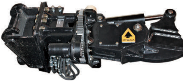
DX-TS-RLS-6in-HX Model 6in (16cm) model for 5-8T excavators 3,000psi cylinder ram.
